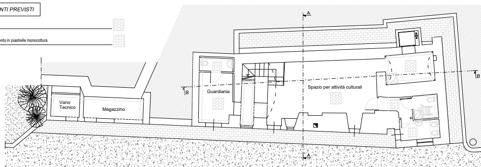
PIANO TERRA
